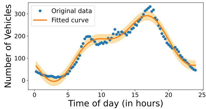
Figure 3.2: Representation of averaged ground truth vehicle counts and generated traffic flow model. To ensure variance in generated vehicle counts, a small deviation \alpha is considered.
