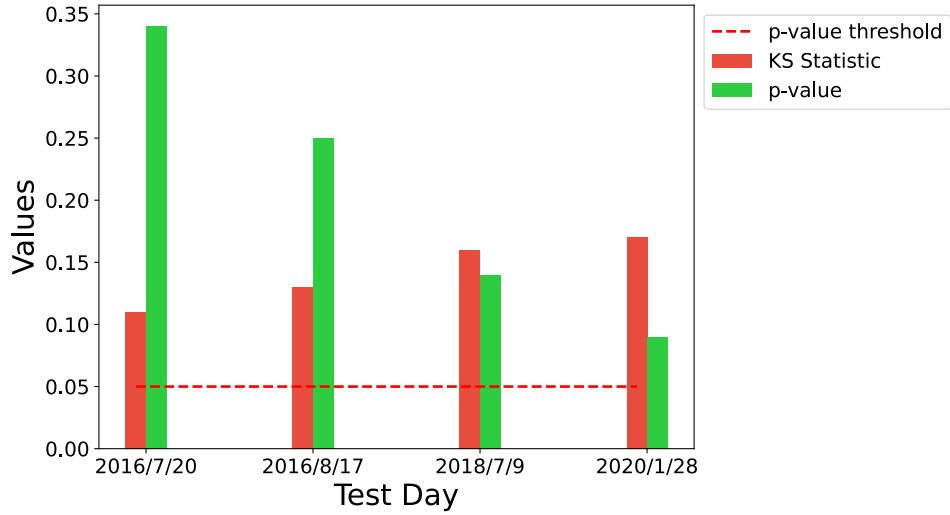
Figure 5.1: The KS Statistic and the p-value obtained from the KS test for the four days of data made available by Tempe are shown. The p-value threshold is indicated as the red line.
