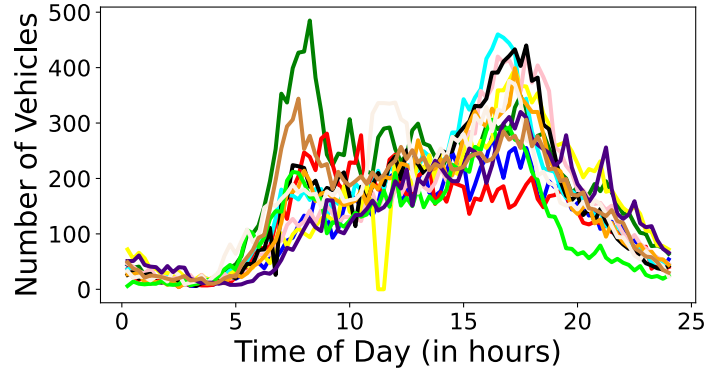
Figure 3.1: The plot of the vehicle counts for a 24-hour period from the Department of Transportation of Tempe for the 12 roads between the placed sensors of interest from the selected Tempe region shown in Fig. 3.3.
