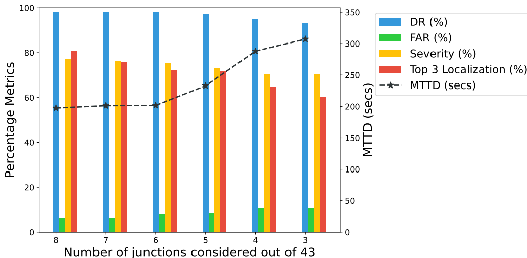
Figure 5.2: Our approaches’ performance with consideration for different sparsity levels. Notice that the incident detection rate is still high for sparsity, as high as 93%. Tabnet performs better in incident detection with a low false alarm rate.
