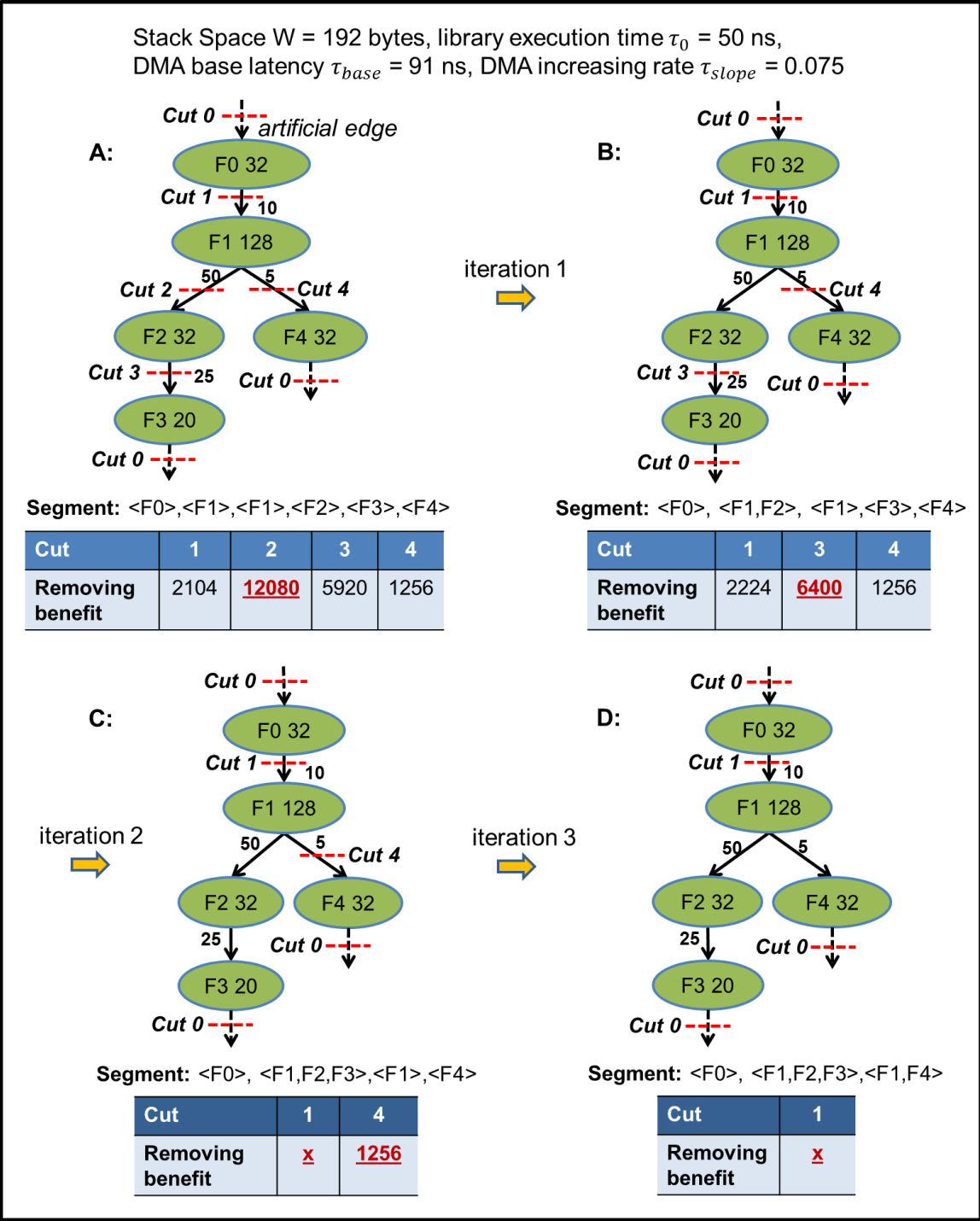
Figure 6.4: Illustration of SSDM heuristic: the values on edges are the numbers of function calls.
