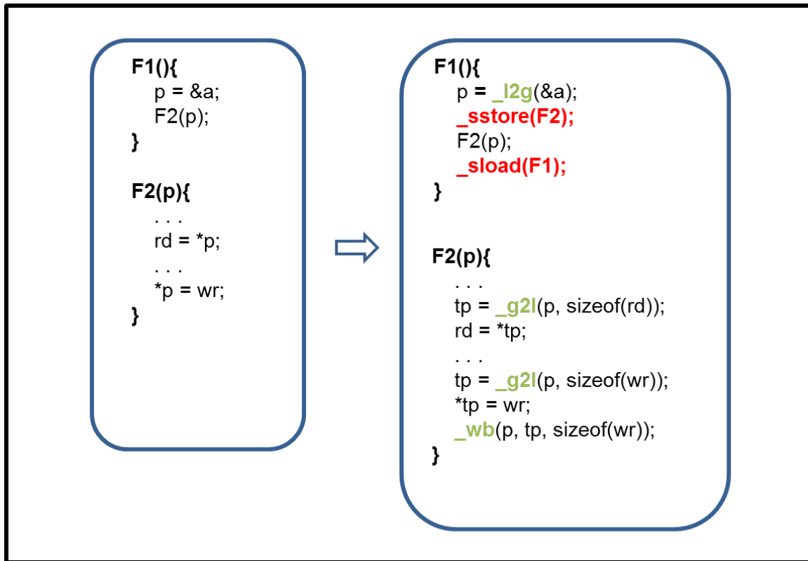
Figure 6.8: Pointer Management - Function F2 accesses the pointer p , which points to a local variable 'a' of function F1. Since 'a' is a local variable on the stack of F1, it has a local address. When F2 is called, if F1 is evicted from the local memory, then the pointer p will point to a wrong value. This is fixed by assigning a global address to the pointer when it is created (through _l2g ), and then when needed, it is accessed through _g2l . Finally it is written back using _wb .
